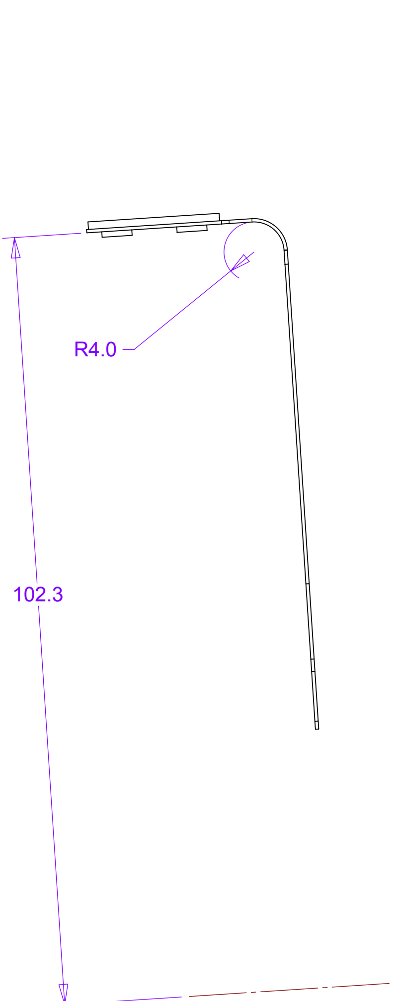
VIEW B-B
